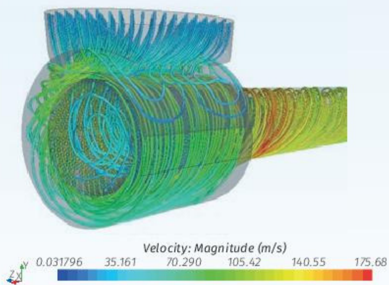
Flow trajectories in SuperTornado™ mixing chamber.
